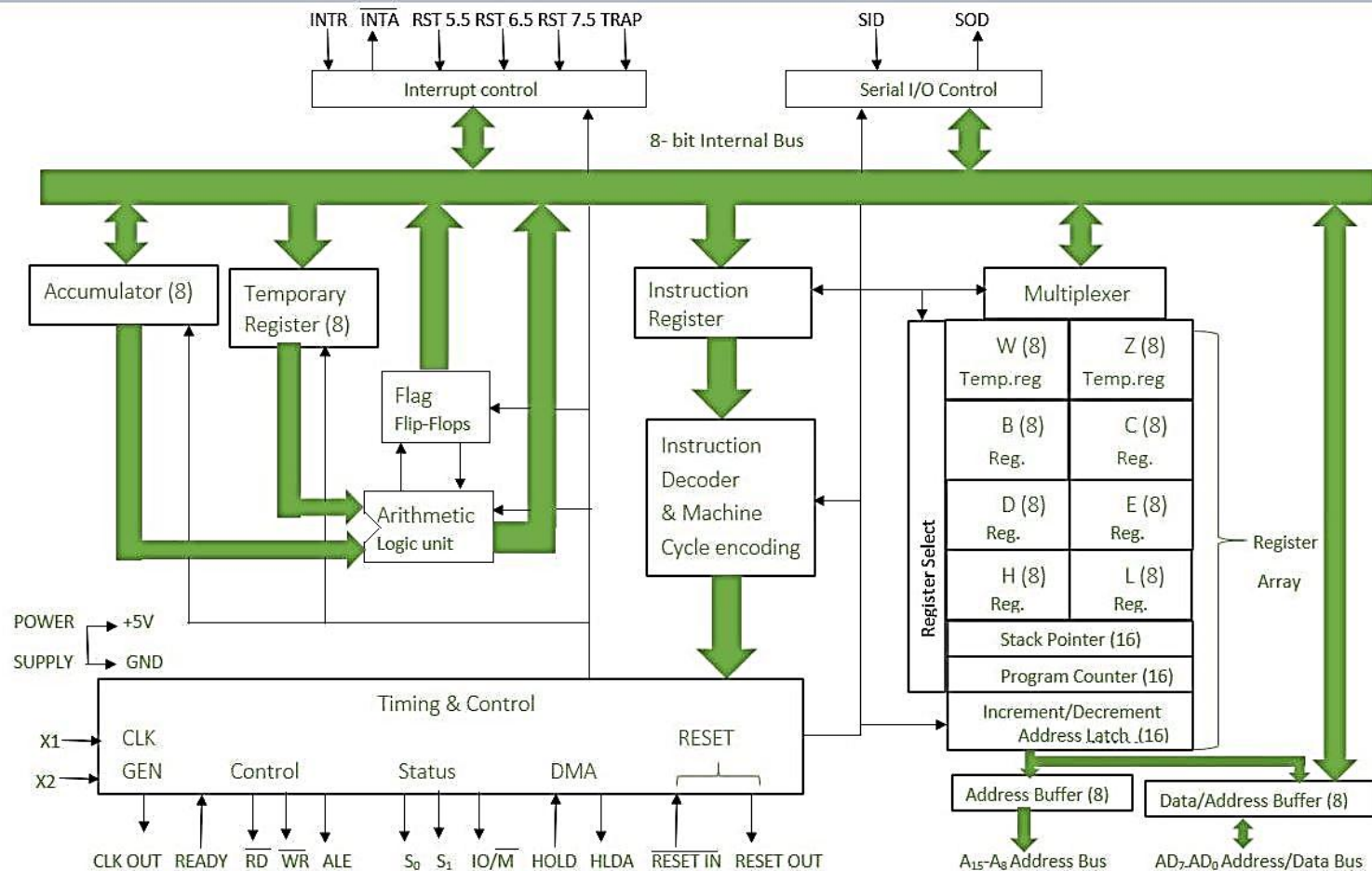
8085 Microprocessor Architecture
